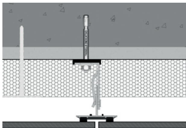
VERTICAL SECTION
